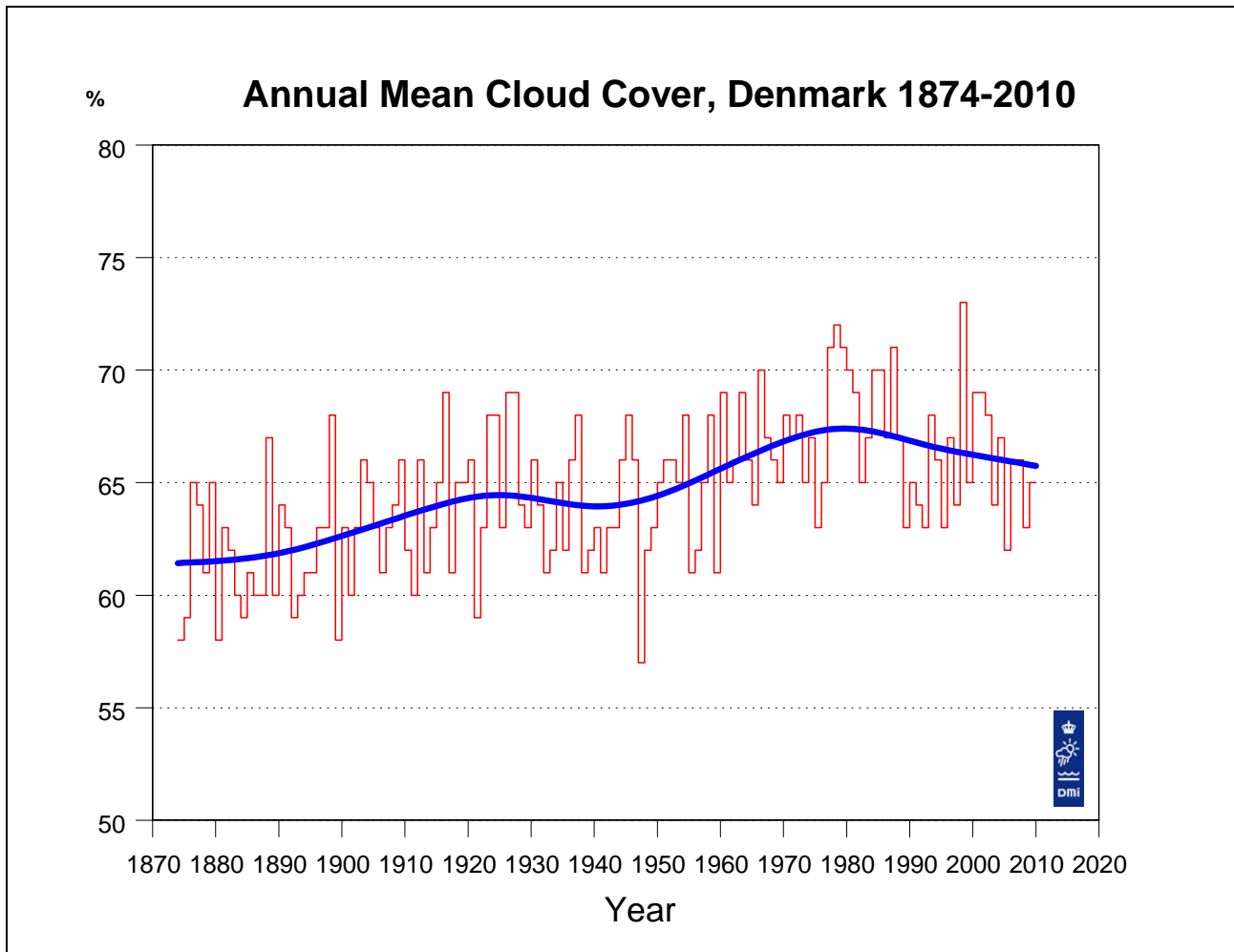
Figure 7. Annual mean cloud cover, Denmark 1874-2010. A Gauss filter with filter width (standard deviation) 9 years has been used to create the “bold” smooth curve. A Gauss filter with standard deviation 9 years is comparable to a 30-years running mean. However, the filter gives a smoother curve than a running mean, as cloud cover values from central years are given larger weight than cloud cover values from periferal years. Filter values are also calculated for the years at either end of the series. It should be noted that these values are computed from one-sided Gauss filters, and that values from later years will change when the series is updated.
