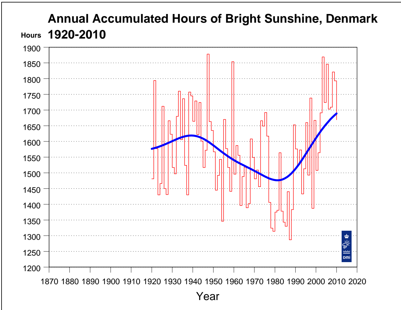
Figure 6. Annual accumulated hours of bright sunshine, Denmark 1920-2010. A Gauss filter with filter width (standard deviation) 9 years has been used to create the “bold” smooth curve. A Gauss filter with standard deviation 9 years is comparable to a 30-years running mean. However, the filter gives a smoother curve than a running mean, as sunshine values from central years are given larger weight than sunshine values from periferal years. Filter values are also calculated for the years at either end of the series. It should be noted that these values are computed from one-sided Gauss filters, and that values from later years will change when the series is updated.
