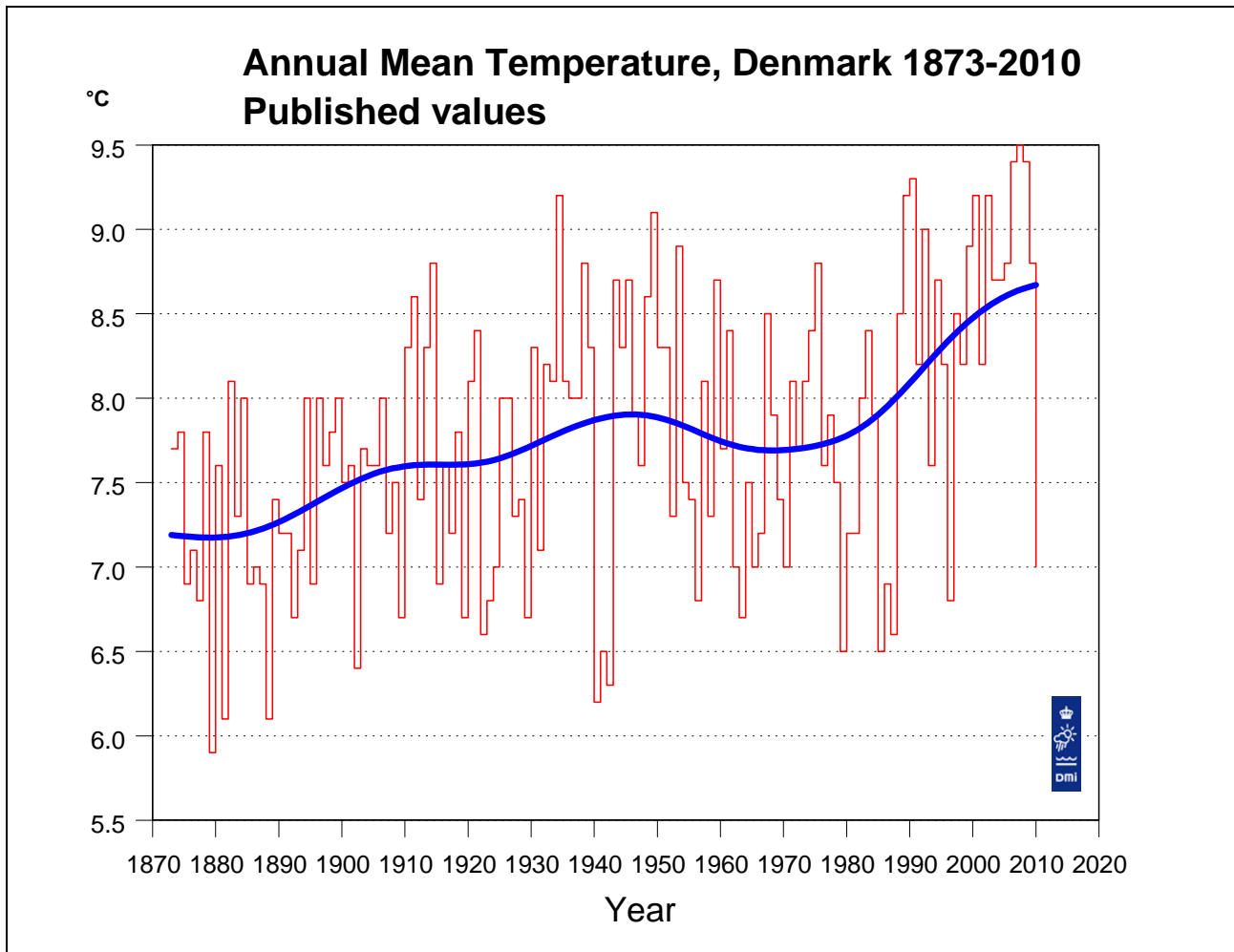
Figure 3. Annual mean temperature, Denmark 1873-2010, published values. A Gauss filter with filter width (standard deviation) 9 years has been used to create the “bold” smooth curve. A Gauss filter with standard deviation 9 years is comparable to a 30-years running mean. However, the filter gives a smoother curve than a running mean, as temperature values from central years are given larger weight than temperature values from peripheral years. Filter values are also calculated for the years at either end of the series. It should be noted that these values are computed from one-sided Gauss filters, and that values from later years will change when the series is updated.
