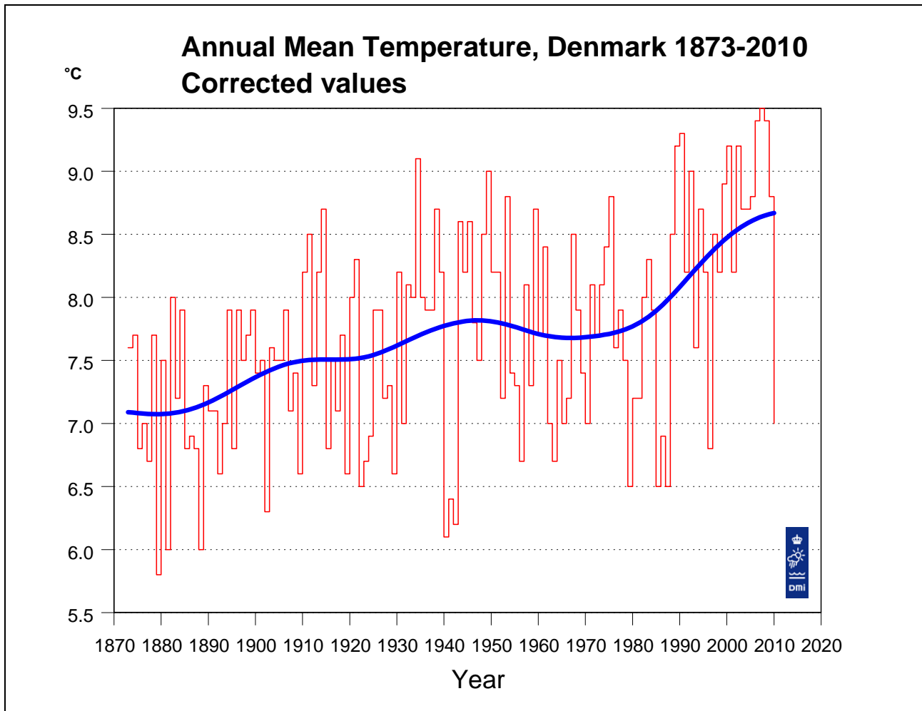
Figure 4. Annual mean temperature, Denmark 1873-2010, corrected values. A Gauss filter with filter width (standard deviation) 9 years has been used to create the “bold” smooth curve. A Gauss filter with standard deviation 9 years is comparable to a 30-years running mean. However, the filter gives a smoother curve than a running mean, as temperature values from central years are given larger weight than temperature values from periferal years. Filter values are also calculated for the years at either end of the series. It should be noted that these values are computed from one-sided Gauss filters, and that values from later years will change when the series is updated.
