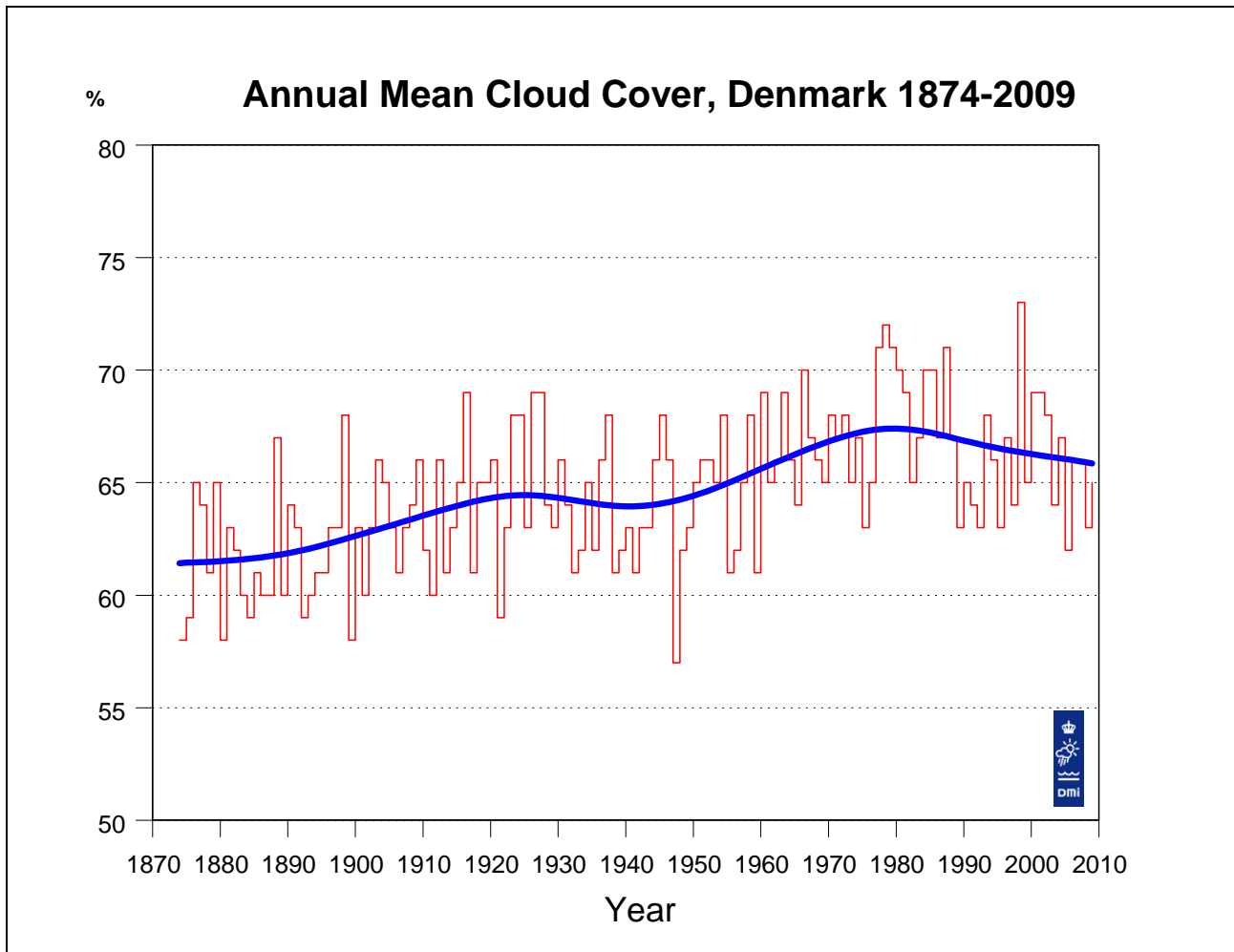
Figure 7. Annual mean cloud cover, Denmark 1874-2009. A Gauss filter with filter width (standard deviation) 9 years has been used to create the “bold” smooth curve. A Gauss filter with standard deviation 9 years is comparable to a 30-years running mean. However, the filter gives a smoother curve than a running mean, as cloud cover values from central years are given larger weight than cloud cover values from periferal years. Filter values are also calculated for the years at either end of the series. It should be noted that these values are computed from one-sided Gauss filters, and that values from later years will change when the series is updated.
