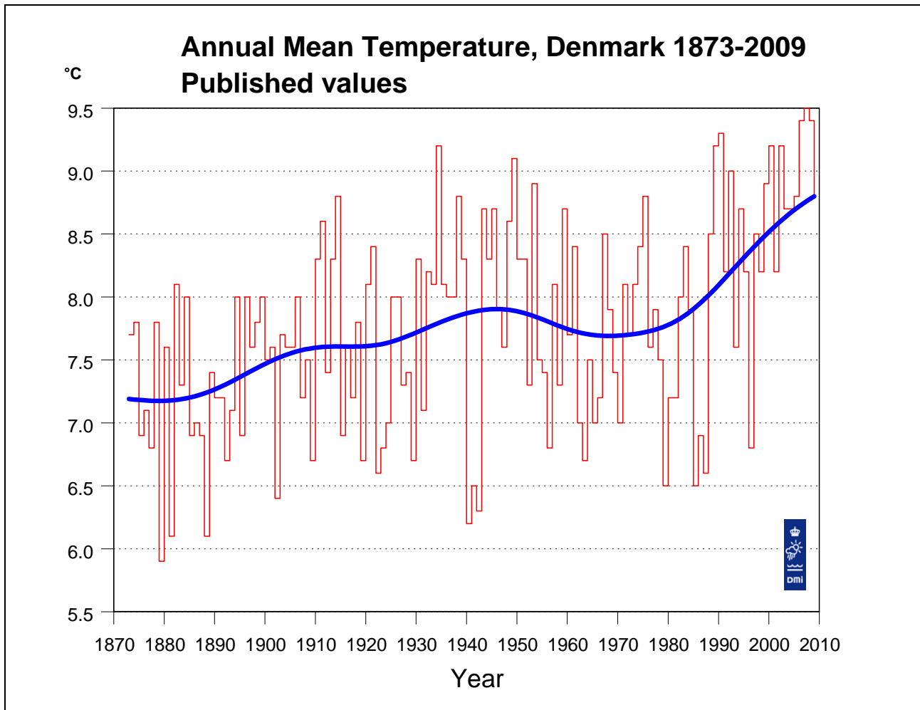
Figure 3. Annual mean temperature, Denmark 1873-2009, published values. A Gauss filter with filter width (standard deviation) 9 years has been used to create the “bold” smooth curve. A Gauss filter with standard deviation 9 years is comparable to a 30-years running mean. However, the filter gives a smoother curve than a running mean, as temperature values from central years are given larger weight than temperature values from periferal years. Filter values are also calculated for the years at either end of the series. It should be noted that these values are computed from one-sided Gauss filters, and that values from later years will change when the series is updated.
