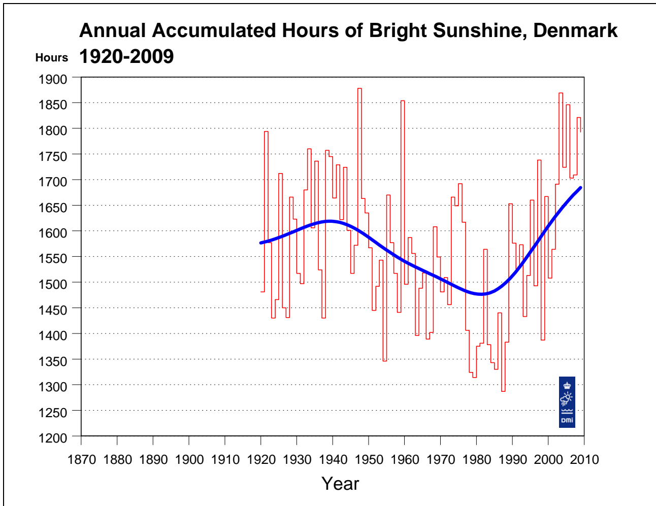
Figure 6. Annual accumulated hours of bright sunshine, Denmark 1920-2009. A Gauss filter with filter width (standard deviation) 9 years has been used to create the “bold” smooth curve. A Gauss filter with standard deviation 9 years is comparable to a 30-years running mean. However, the filter gives a smoother curve than a running mean, as sunshine values from central years are given larger weight than sunshine values from periferal years. Filter values are also calculated for the years at either end of the series. It should be noted that these values are computed from one-sided Gauss filters, and that values from later years will change when the series is updated.
