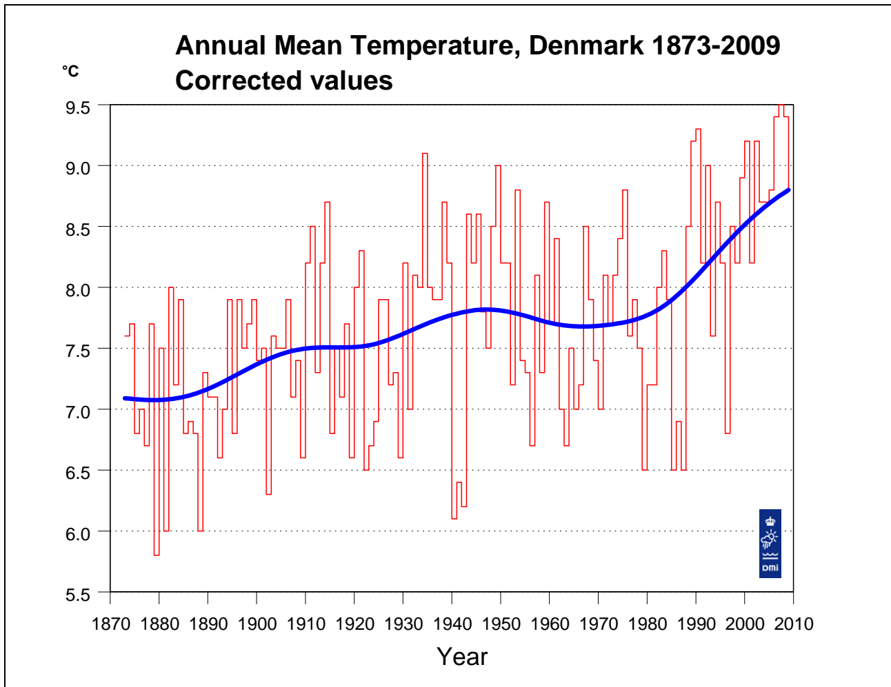
Figure 4. Annual mean temperature, Denmark 1873-2009, corrected values. A Gauss filter with filter width (standard deviation) 9 years has been used to create the “bold” smooth curve. A Gauss filter with standard deviation 9 years is comparable to a 30-years running mean. However, the filter gives a smoother curve than a running mean, as temperature values from central years are given larger weight than temperature values from periferal years. Filter values are also calculated for the years at either end of the series. It should be noted that these values are computed from one-sided Gauss filters, and that values from later years will change when the series is updated.
