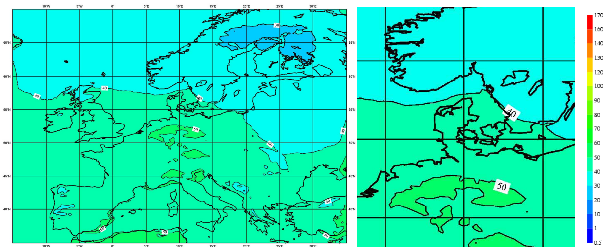
Figure 11: Averaged annual ozone concentration (in \mu\text{g}/\text{m}^3 ) for year of 2000 (simulated by HIRLAM+CAMx).
