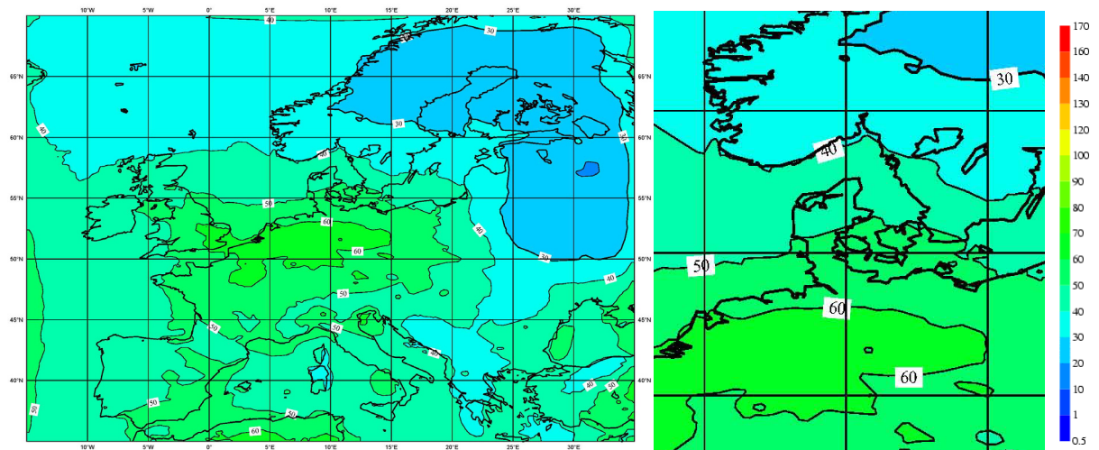
Figure 8: Averaged seasonal ozone concentration (in \mu\text{g}/\text{m}^3 ) for summer 2000 (simulated by HIRLAM+CAMx).
