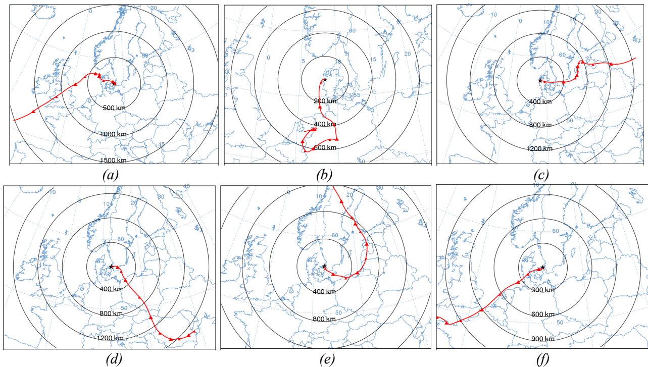
Figure 3: Backward trajectories (calculated by the NOAA HYSPLIT model) showing atmospheric transport from the (a) South-Western sector arrived at DK41 on 30 Jul 1994, 15 UTC; (b) Southern sector arrived at DK31 on 6 Jun 1996, 18 UTC; (c) Eastern sector arrived at DK31 on 2 Jun 1992, 14 UTC; (d) South-Eastern sector arrived at DK32 on 28 Apr 1993, 12 UTC; (e) Southern sector arrived at DK32 on 13 May 1993, 15 UTC, (f) South-Western sector arrived at DK32 on 28 Jul 1994, 11 UTC.
