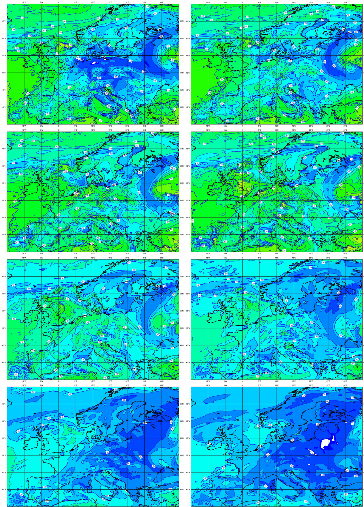
Figure B3: Ozone concentration (in \mu\text{g}/\text{m}^3 ) field for 21 Jun 2000 (03, 06, 09, 12, 15, 18, 21, 24 UTC) (simulated by HIRLAM+CAMx).
