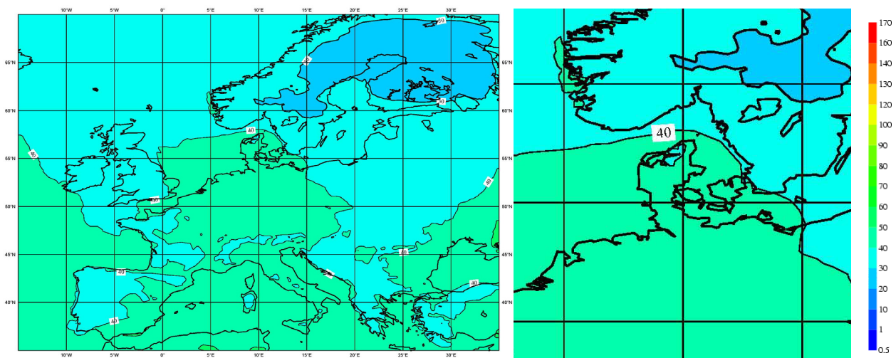
Figure 9: Averaged seasonal ozone concentration (in \mu\text{g}/\text{m}^3 ) for fall 2000 (simulated by HIRLAM+CAMx).
