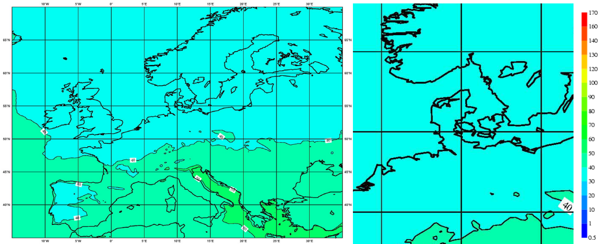
Figure 10: Averaged seasonal ozone concentration (in \mu\text{g}/\text{m}^3 ) for winter 2000 (simulated by HIRLAM+CAMx).
