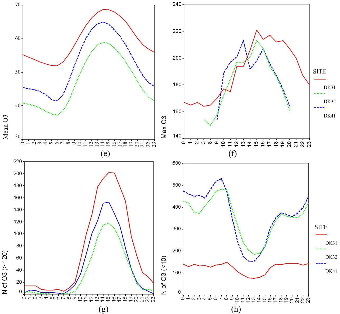
Figure 2 : Ozone inter-annual (a,b), monthly (c,d) and diurnal cycle (e,f,g,h) variability for the mean concentration in \mu\text{g}/\text{m}^3 (a,c,e), absolute maximum concentration (f), number of cases with concentrations below 10 \mu\text{g}/\text{m}^3 (b, h) and above 120 \mu\text{g}/\text{m}^3 (d, g) for three Danish sites DK31, DK32, and DK41.
