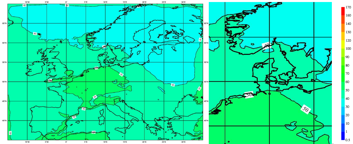
Figure 7: Averaged seasonal ozone concentration (in \mu\text{g}/\text{m}^3 ) for spring 2000 (simulated by HIRLAM+CAMx).
