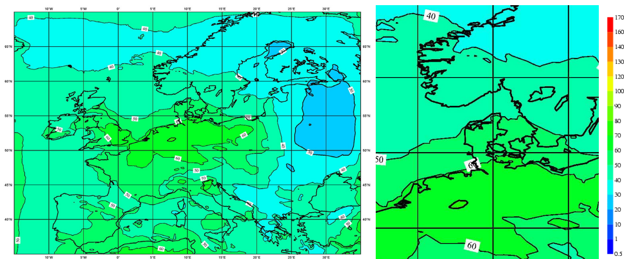
Figure 6: Averaged monthly ozone concentration (in \mu\text{g}/\text{m}^3 ) for June 2000 (simulated by HIRLAM+CAMx).
