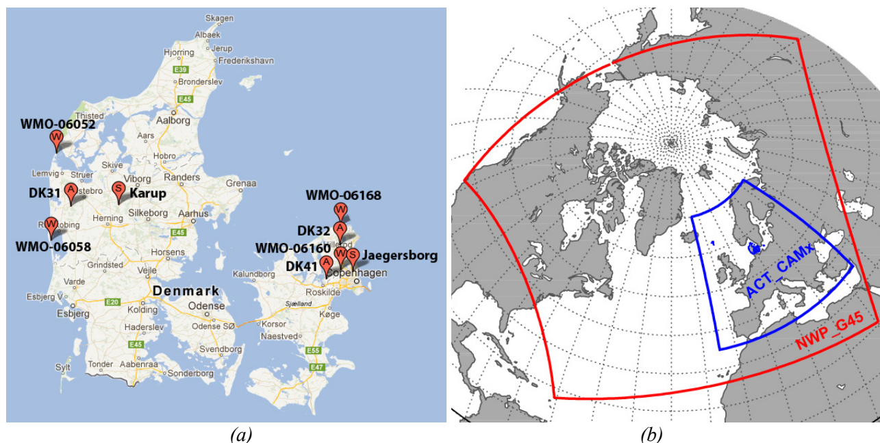
Figure 1: (a) Geographical positions (extracted from Google-Earth) of Danish sites for ozone measurements (A: DK31, DK32, and DK41), synoptical meteorological stations (W: WMO-06160 – Vaerlose, WMO-06168 – Nakkehoved Fyr, WMO-06058 – Hvide Sande, WMO-06052 – Thyboron) and sounding stations (S: Jaegersborg, Karup); and (b) Boundaries of domains for atmospheric (NWP_G45) and chemical transport (ACT-CAMx) modelling.
