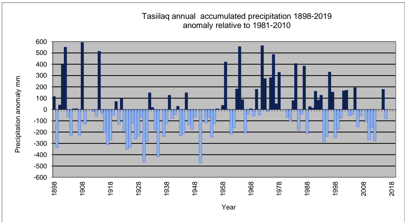
Annual accumulated precipitation since 1898 for 4360 Tasillaq; anomaly relative to 1981-2010. There are missing values for some years 1910-1911, 1936, 1949, 1951, 1979-1980, 2008, 2013-2014 and 2017-2019.
