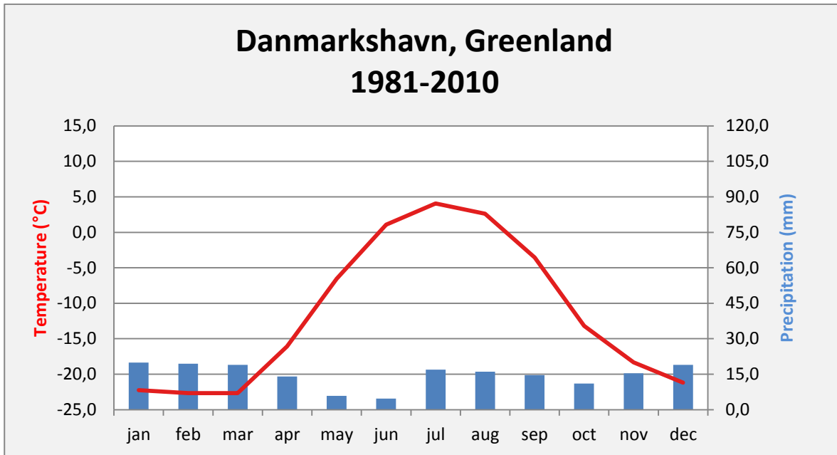
Annual average air temperature and annual accumulated precipitation for 4320 Danmarkshavn 1981-2010.
