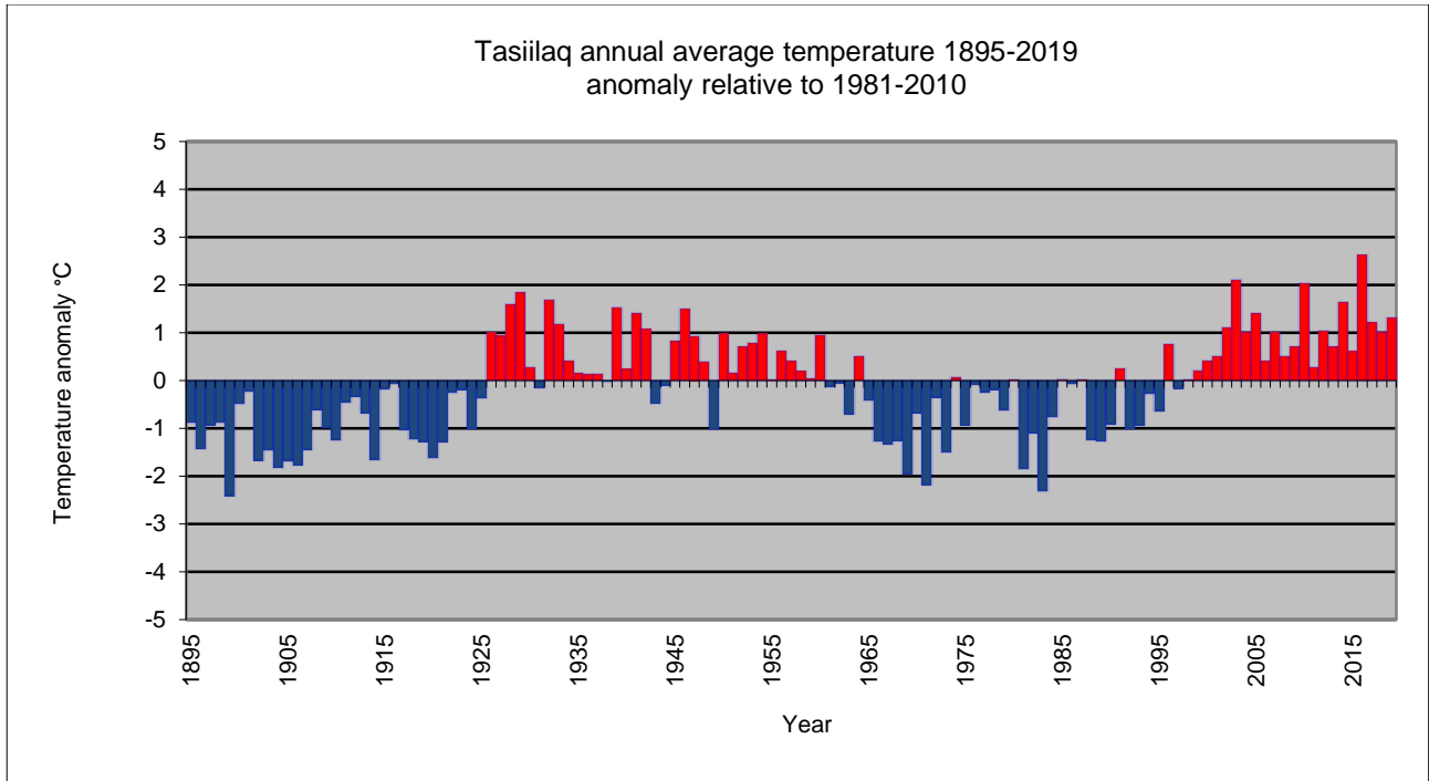
Annual average air temperature since 1895 for 4360 Tasillaq; anomaly relative to 1981-2010.
