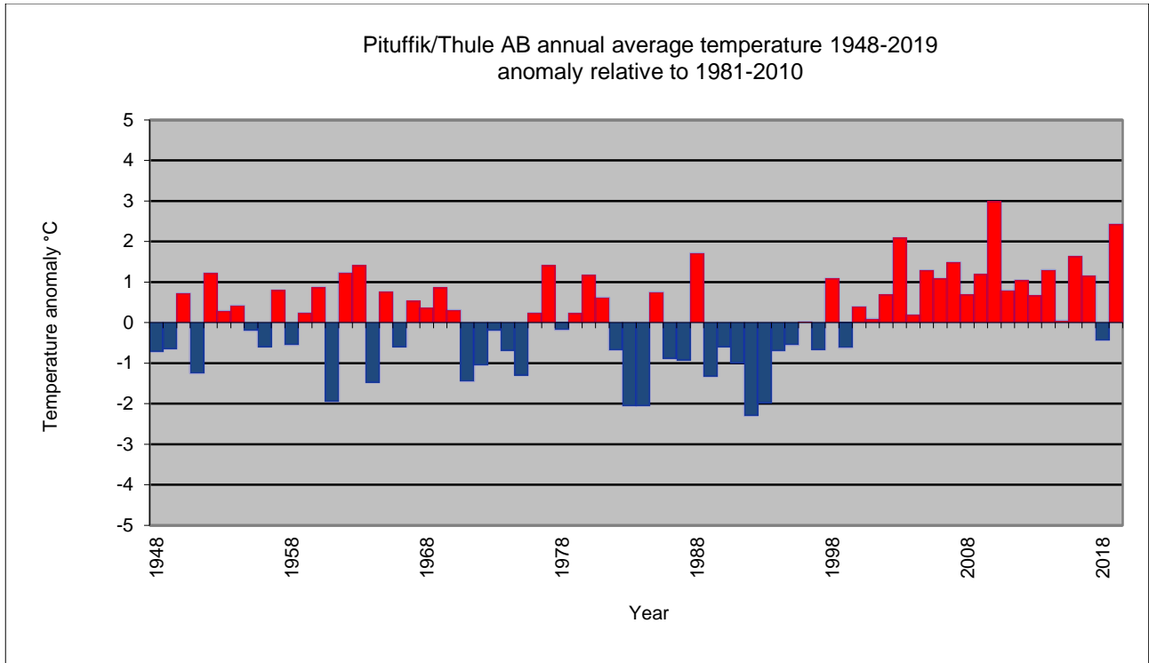
Annual average air temperature since 1948 for 4202 Pituffik/Thule AB; anomaly relative to 1981-2010.
