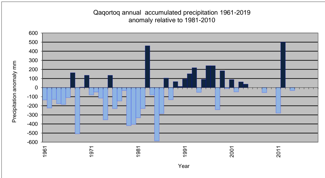
Annual accumulated precipitation since 1961 for 4272 Qaqortoq; anomaly relative to 1981-2010. There are missing values for some years 2005-2007, 2009-2010, 2013 and 2015-2019.
