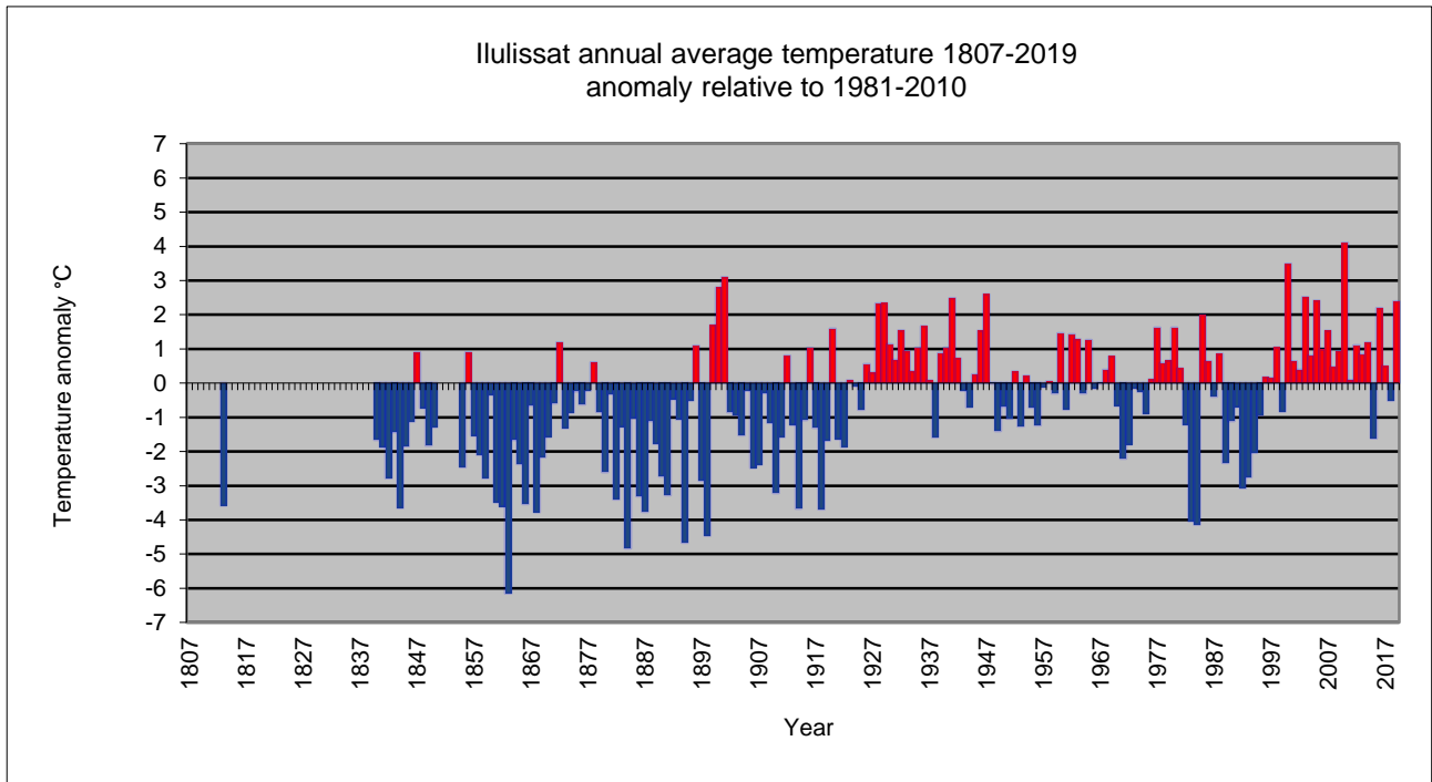
Annual average air temperature since 1807 for 4221 Ilulissat; anomaly relative to 1981-2010. There are missing values for some early years 1807-1812, 1814-1838 and 1851-1854.
