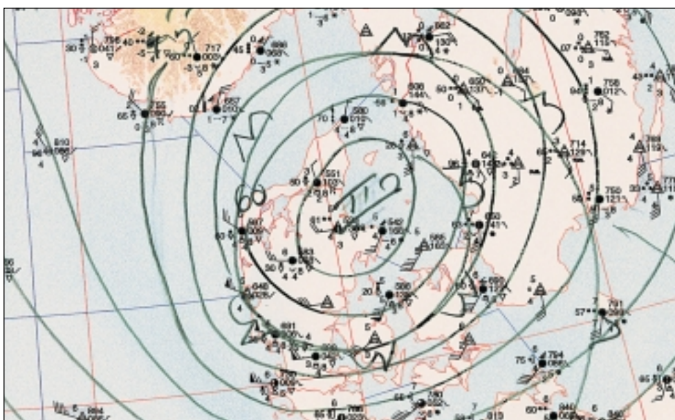
The hurricane on 3 December 1999 resulted in the highest wind speeds ever recorded in Denmark – 38 metres per second. The hurricane caused several fatalities and property damage exceeding 2 billion euro.
