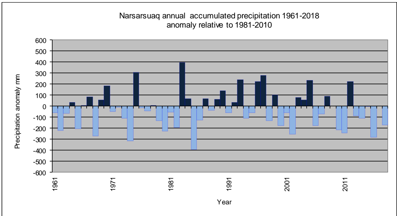
Annual accumulated precipitation since 1961 for 4270 Narsarsuaq; anomaly relative to 1981-2010. There are missing values for one year 2009.
