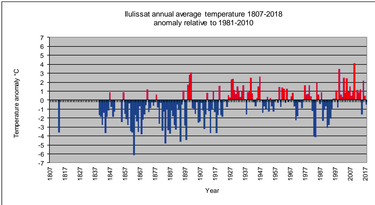
Figure 7.2.3. Top: Annual average air temperature since 1807 for 4221 Ilulissat; anomaly relative to 1981-2010 (shown as graph and table in the bottom).
