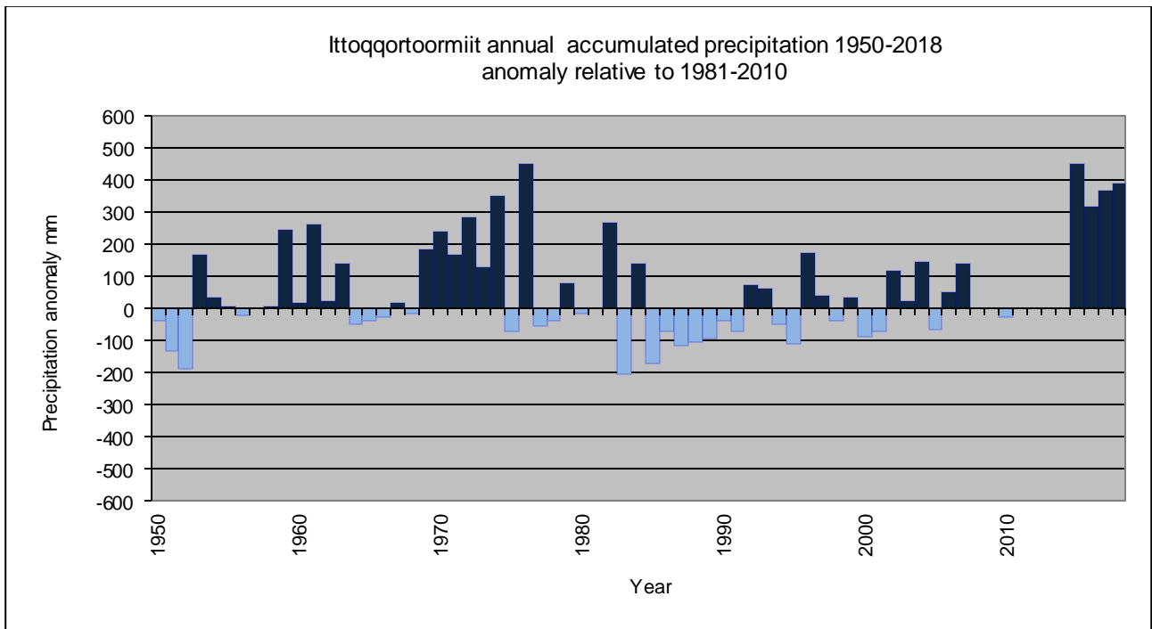
Annual accumulated precipitation since 1950 for 4339 Ittoqqortoormiit; anomaly relative to 1981-2010. There are missing values for some years 1957, 1981, 2008-2009 and 2011-2014.
