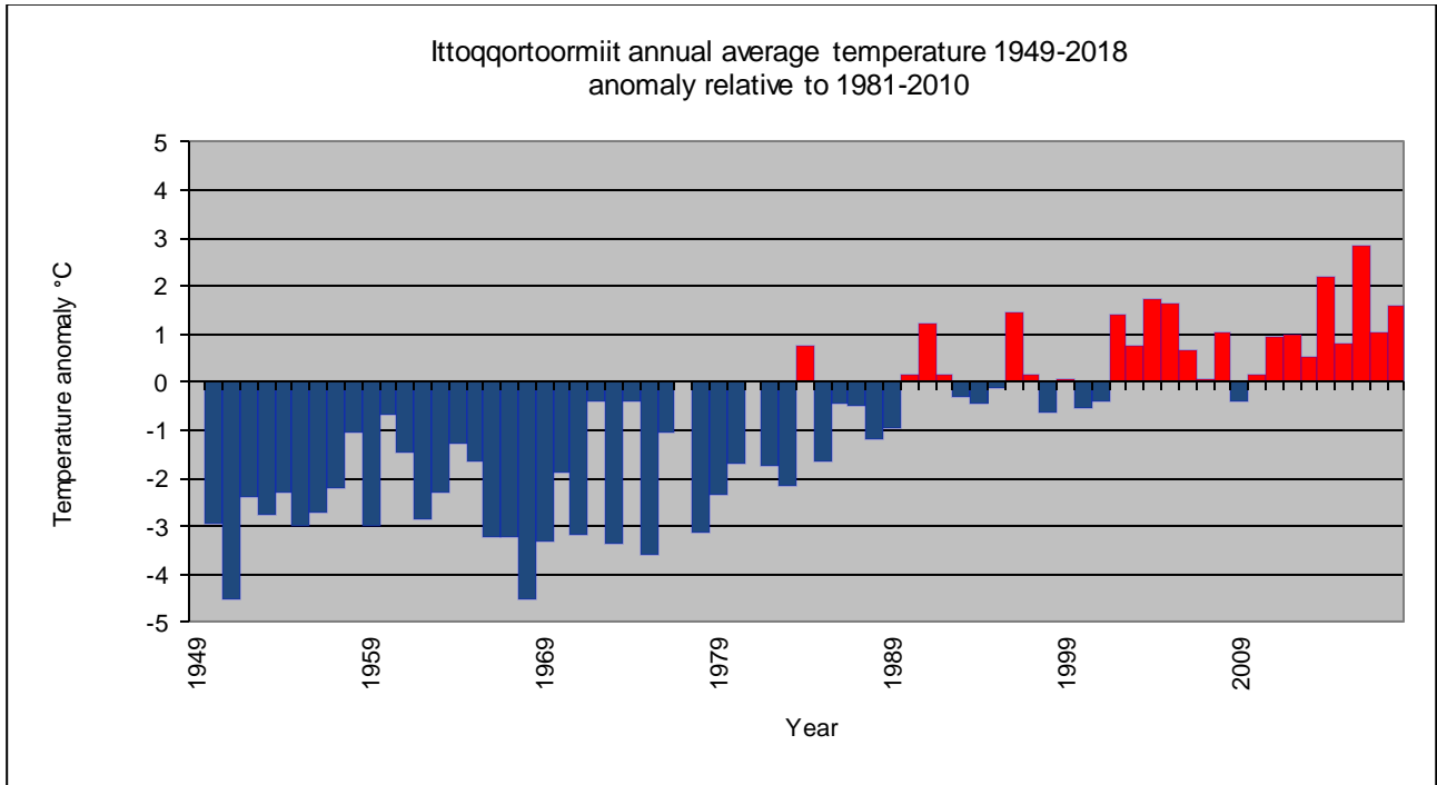
Annual average air temperature since 1949 for 4339 Ittoqqortoormiit; anomaly relative to 1981-2010. There are missing values for some years 1949, 1977 and 1981.
