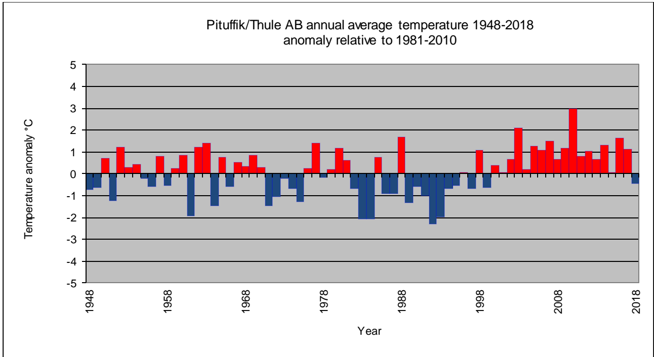
Annual average air temperature since 1948 for 4202 Pituffik/Thule AB; anomaly relative to 1981-2010.
