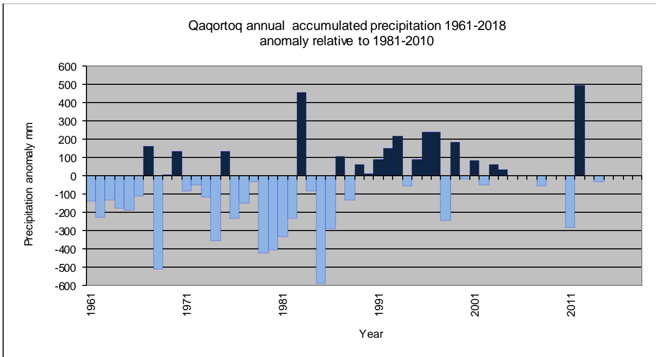
Annual accumulated precipitation since 1961 for 4272 Qaqortoq; anomaly relative to 1981-2010. There are missing values for some years 2005-2007, 2009-2010, 2013 and 2015-2018.
