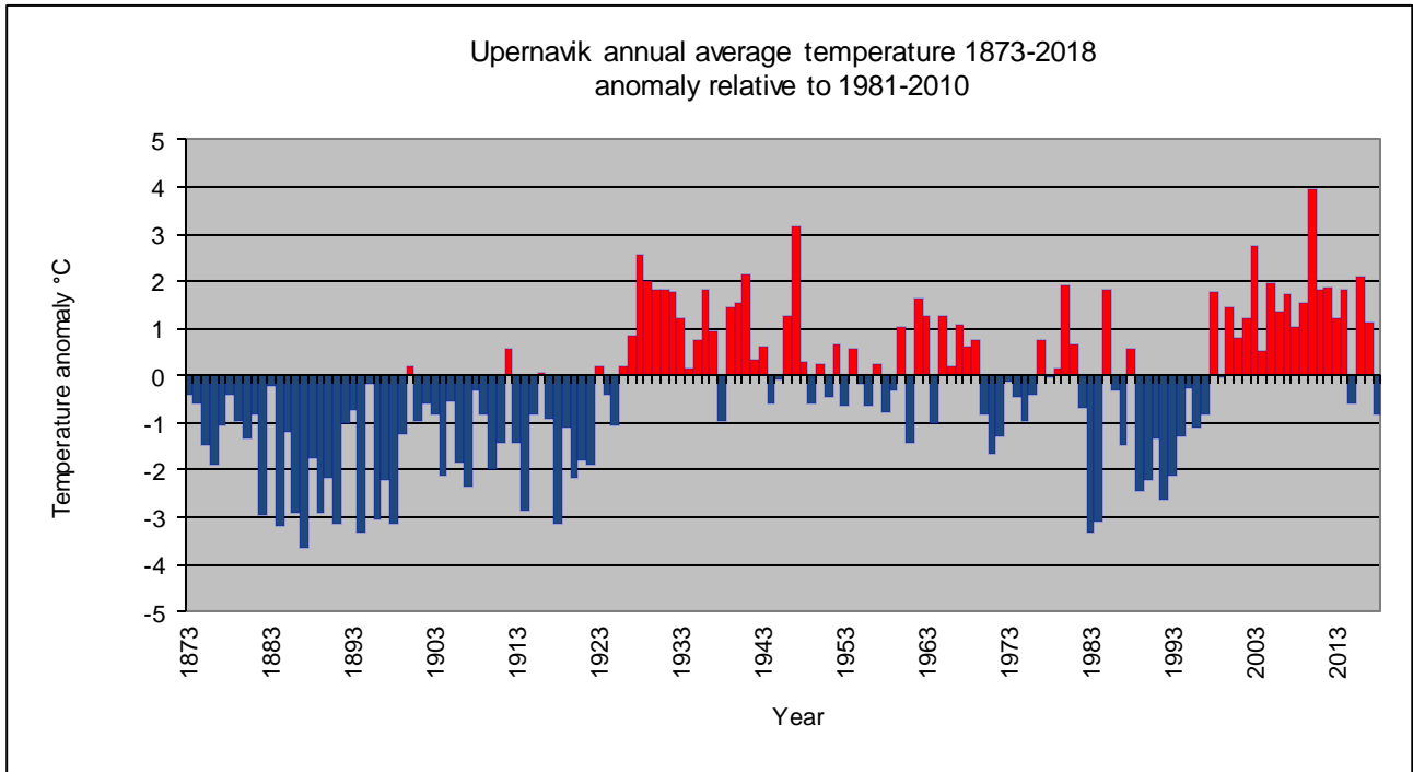
Annual average air temperature since 1873 for 4211 Upernavik; anomaly relative to 1981-2010.
