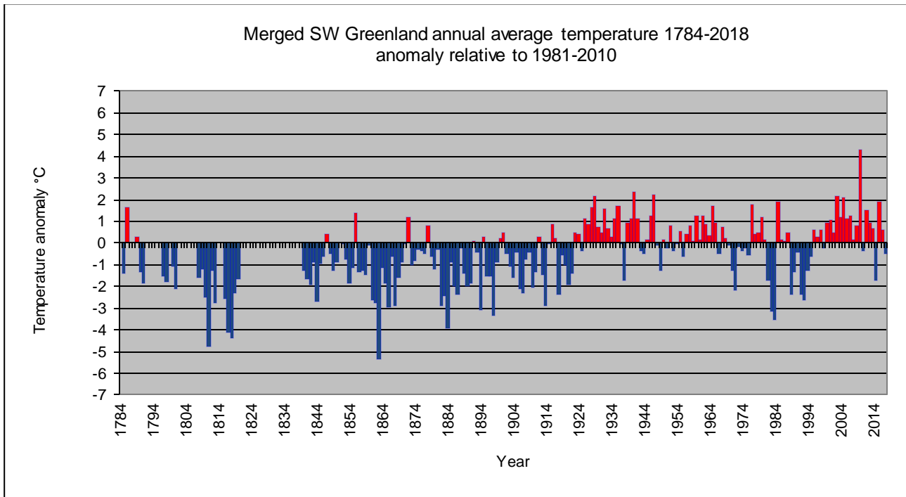
Figure 7.2.10. Annual average air temperature since 1784 for a merged SW Greenland series (see section 6.2.1 and Appendix 4); anomaly relative to 1981-2010. There are missing values for some early years 1784, 1787-1789, 1792-1796, 1799, 1802-1807, 1814-1815, 1821-1839 and 1851.
