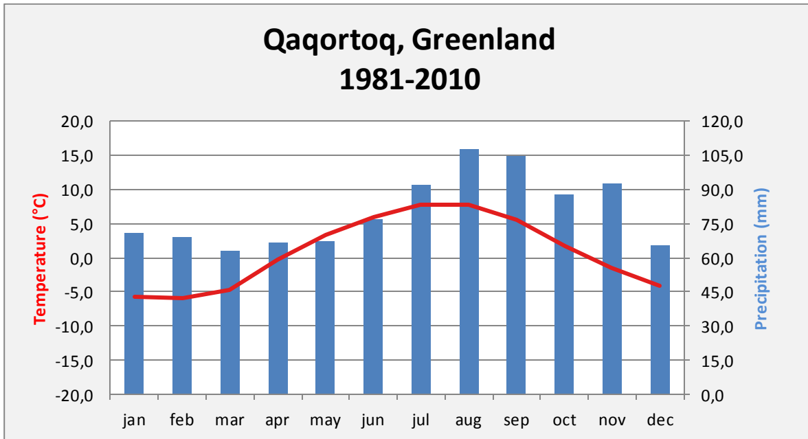
Annual average air temperature and annual accumulated precipitation for 4272 Qaqortoq 1981-2010.
