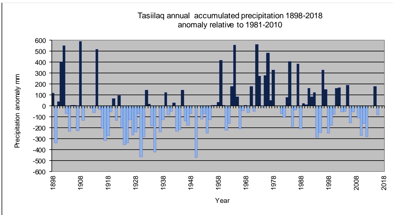
Annual accumulated precipitation since 1898 for 4360 Tasiilaq; anomaly relative to 1981-2010. There are missing values for some years 1910-1911, 1936, 1949, 1951, 1979-1980, 2008, 2013-2014 and 2017-2018.
