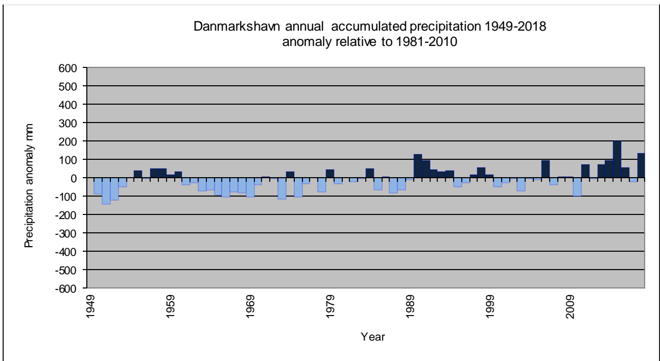
Annual accumulated precipitation since 1949 for 4320 Danmarkshavn; anomaly relative to 1981-2010. There are missing values for some years 1949, 1954, 1977 and 1981.
