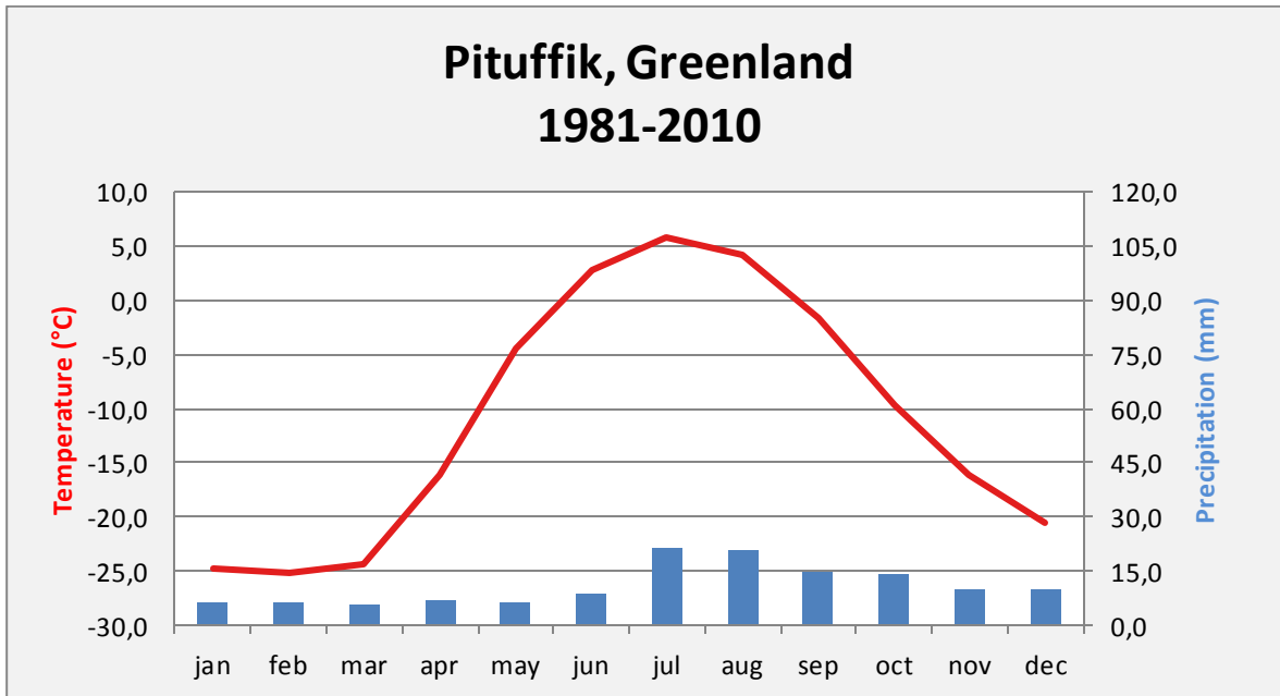
Annual average air temperature and annual accumulated precipitation for 4202 Pituffik/Thule AB 1981-2010.
