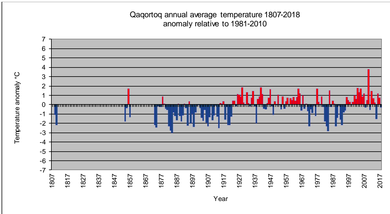
Annual average air temperature since 1807 for 4272 Qaqortoq; anomaly relative to 1981-2010. There are missing values for some early years 1807-1808, 1811-1853 and 1858-1872.
