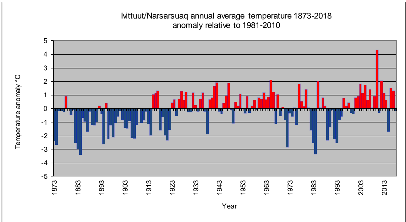
Annual average air temperature since 1873 for 34262/4270 Ivittuut/Narsarsuaq; anomaly relative to 1981-2010.
