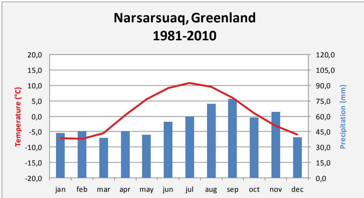
Annual average air temperature and annual accumulated precipitation for 4270 Narsarsuaq 1981-2010.
