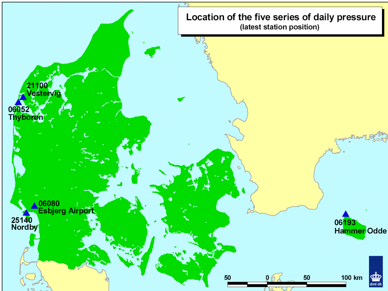
Figure 2.2. Location of the five series of daily air pressure. Together the five series cover three sites with data 1874-2010. The stations representing each site are listed in the table 3.6. For station co-ordinates confer with the station position file in the data files included.
