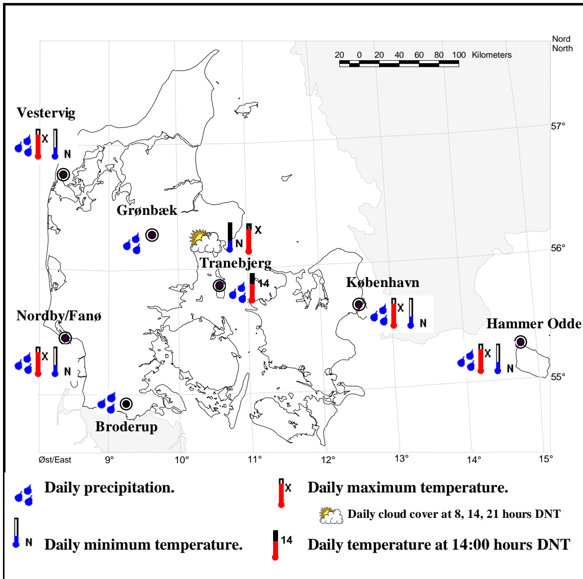
Figure 2.1. The seven Danish sites with digitised daily precipitation, temperature and/or cloud cover observations, 1874-2010. The stations representing each site are listed in the tables 3.1 – 3.5. For station co-ordinates confer with the station position file in the data files included. DNT refers to Danish normal time, which is the time in a given time zone in contrast to summer time, where 1 hour is added. In Denmark the normal time is UTC+1.
