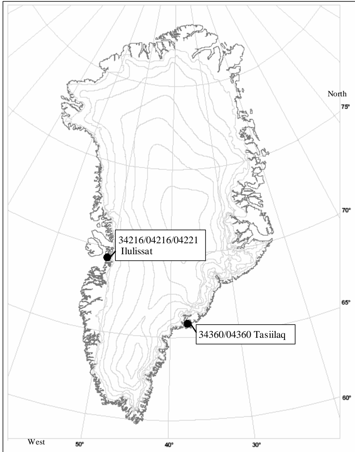
Figure 2.3. The location of the two Greenlandic sites with long daily data series: Ilulissat (formerly: Jacobshavn) on the West Coast and Tasiilaq (formerly: Angmagssalik) on the East Coast, 1873-2010. The stations representing each site are listed in the tables 4.1 – 4.3. For station co-ordinates confer with the station position file in the data files included.
