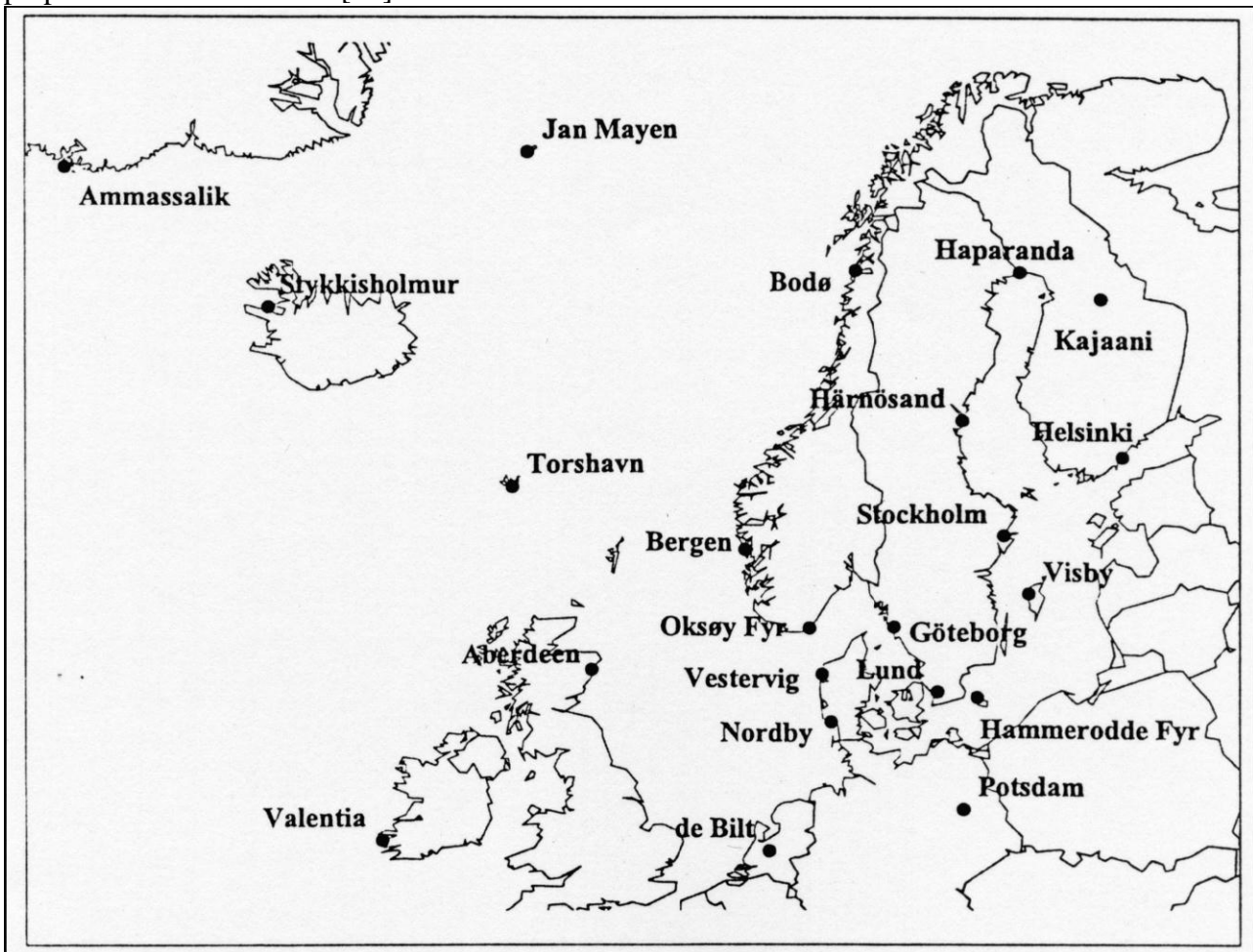
Figure 4.1.1. Location of the stations that originally provided atmospheric pressure observations to the WASA pressure data set [28]. In this report the updated greenlandic series Ammassalik/Tasiilaq is presented. The station representing this site is listed in the table 4.2.1. For station co-ordinates confer with the station position file in the data files included in this report (see Appendix 1). Pressure data sets from Denmark (three sites) and Tórshavn, The Faroe Islands are presented in the representative historical Climate Data Collection; DMI Technical Report 14-02 [13]) and DMI Technical Report 14-05 [14]).
