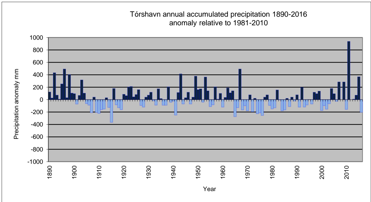
Figure 6.2.2. Annual accumulated precipitation since 1890 for 6011 Tórshavn; anomaly relative to 1981-2010. There are missing values for the years 2008 and 2012.
