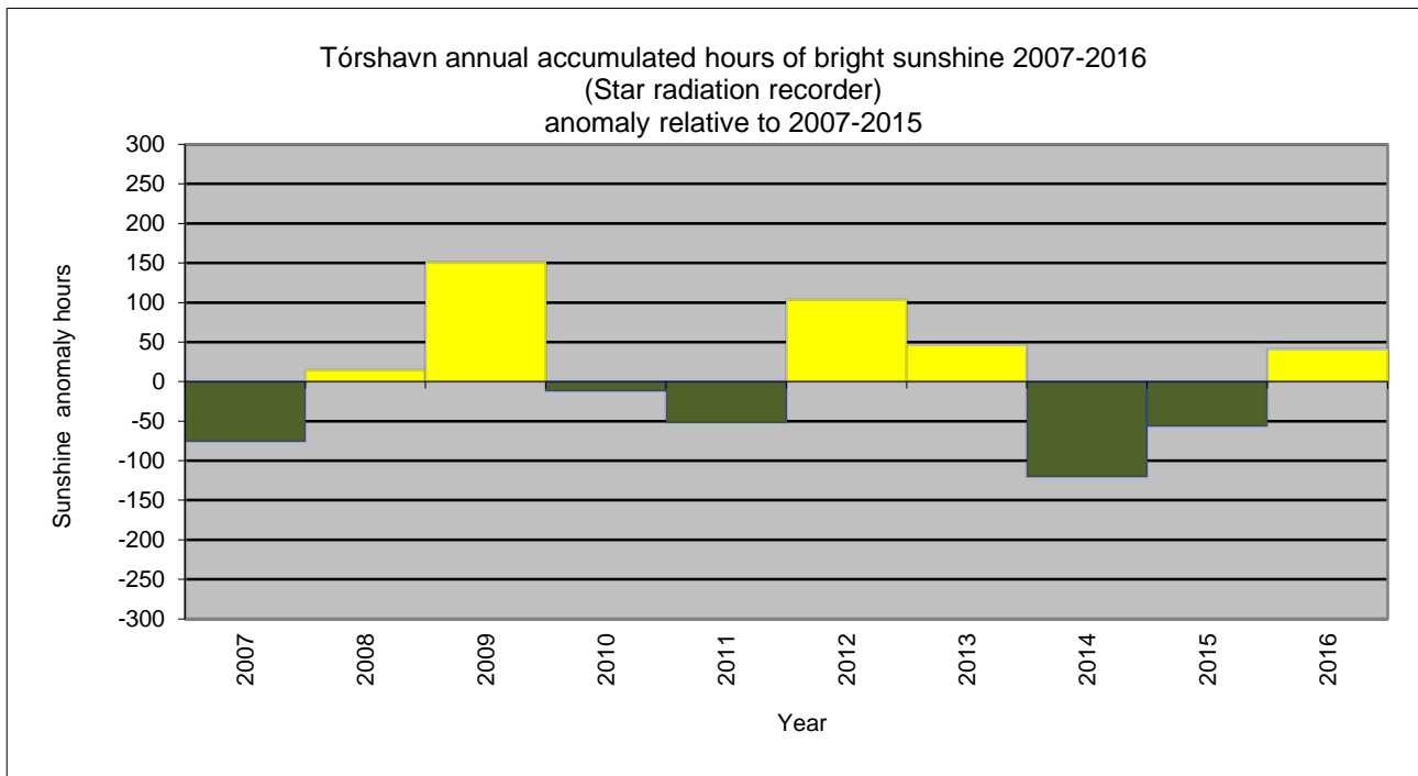
Figure 6.2.4. Annual accumulated hours of bright sunshine 2007-2016 for 6011 Tórshavn; anomaly relative to 2007-2015. The instrument is a Star radiation recorder. OBS! DMI has since 2007 observed the hours of bright sunshine using measurements of global radiation instead of measurements from a traditional Fuess sunshine recorder before. For that reason “new” and “old” hours of bright sunshine cannot directly be compared; see figure above.
