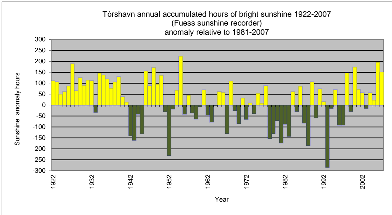
Figure 6.2.3. Annual accumulated hours of bright sunshine 1922-2007 for 33069 Tórshavn Radiosonde; anomaly relative to 1981-2007. The instrument was a Fuess sunshine recorder. OBS! DMI has since 2007 observed the hours of bright sunshine using measurements of global radiation instead of measurements from a traditional Fuess sunshine recorder. For that reason “new” and “old” hours of bright sunshine cannot directly be compared; see figure below.
