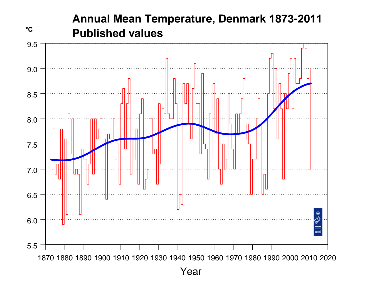
Figure 5.4.1. Annual mean temperature, Denmark 1873-2011, published values. A Gauss filter with filter width (standard deviation) 9 years has been used to create the “bold” smooth curve. A Gauss filter with standard deviation 9 years is comparable to a 30-years running mean. However, the filter gives a smoother curve than a running mean, as temperature values from central years are given larger weight than temperature values from periferal years. Filter values are also calculated for the years at either end of the series. It should be noted that these values are computed from one-sided Gauss filters, and that values from later years will change when the series is updated.
