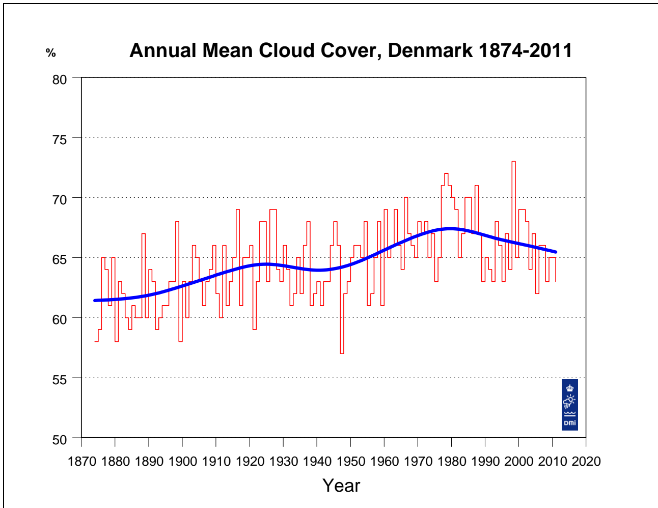
Figure 5.4.4. Annual mean cloud cover, Denmark 1874-2011. A Gauss filter with filter width (standard deviation) 9 years has been used to create the “bold” smooth curve. A Gauss filter with standard deviation 9 years is comparable to a 30-years running mean. However, the filter gives a smoother curve than a running mean, as cloud cover values from central years are given larger weight than cloud cover values from periferal years. Filter values are also calculated for the years at either end of the series. It should be noted that these values are computed from one-sided Gauss filters, and that values from later years will change when the series is updated.
