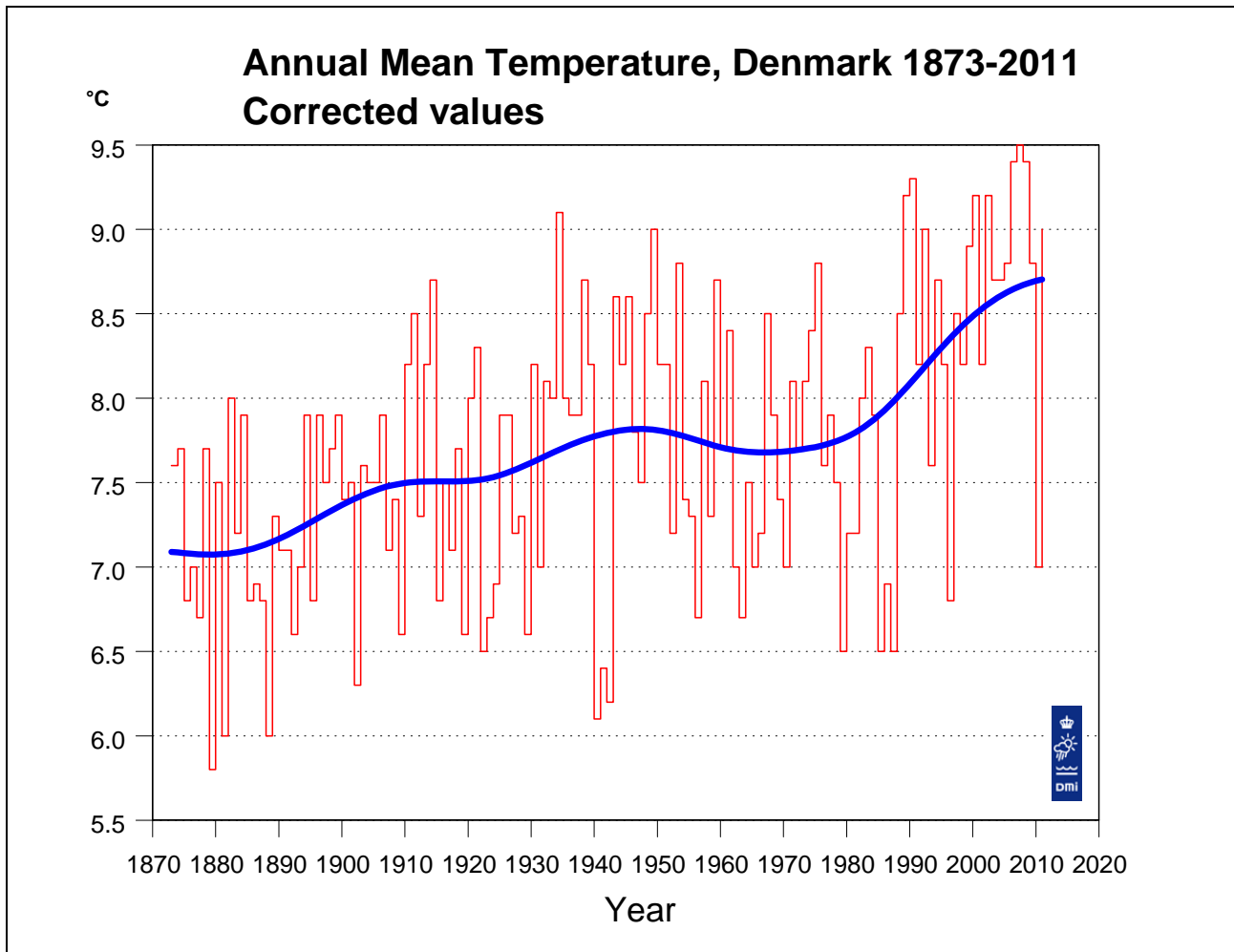
Figure 5.4.2. Annual mean temperature, Denmark 1873-2011, corrected values. A Gauss filter with filter width (standard deviation) 9 years has been used to create the “bold” smooth curve. A Gauss filter with standard deviation 9 years is comparable to a 30-years running mean. However, the filter gives a smoother curve than a running mean, as temperature values from central years are given larger weight than temperature values from periferal years. Filter values are also calculated for the years at either end of the series. It should be noted that these values are computed from one-sided Gauss filters, and that values from later years will change when the series is updated.
