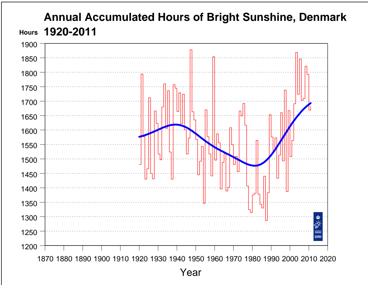
Figure 5.4.3. Annual accumulated hours of bright sunshine, Denmark 1920-2011. A Gauss filter with filter width (standard deviation) 9 years has been used to create the “bold” smooth curve. A Gauss filter with standard deviation 9 years is comparable to a 30-years running mean. However, the filter gives a smoother curve than a running mean, as sunshine values from central years are given larger weight than sunshine values from periferal years. Filter values are also calculated for the years at either end of the series. It should be noted that these values are computed from one-sided Gauss filters, and that values from later years will change when the series is updated.
